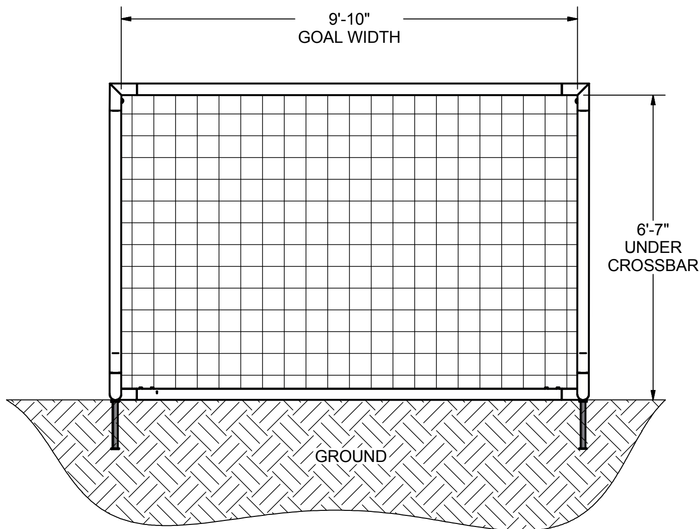
FRONT VIEW
