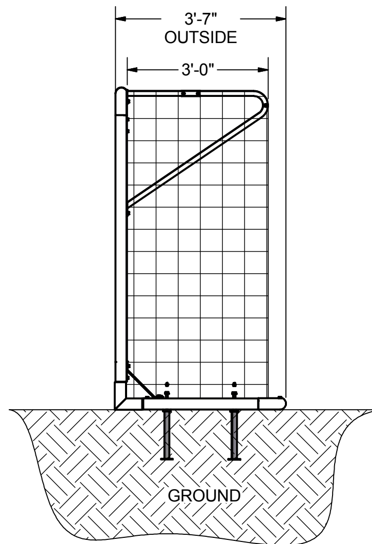
SIDE VIEW
